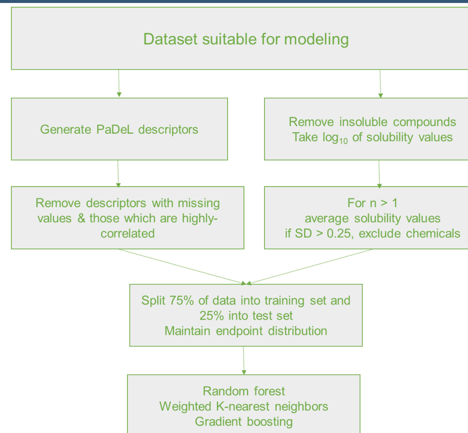
Figure 2 (above): This diagram shows the simplified workflow used in the modeling of the water solubility dataset.
